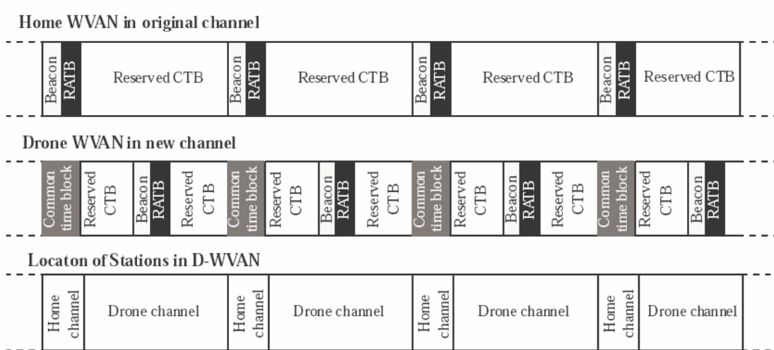
Figure 18: Common time block allocation in D-WVAN
