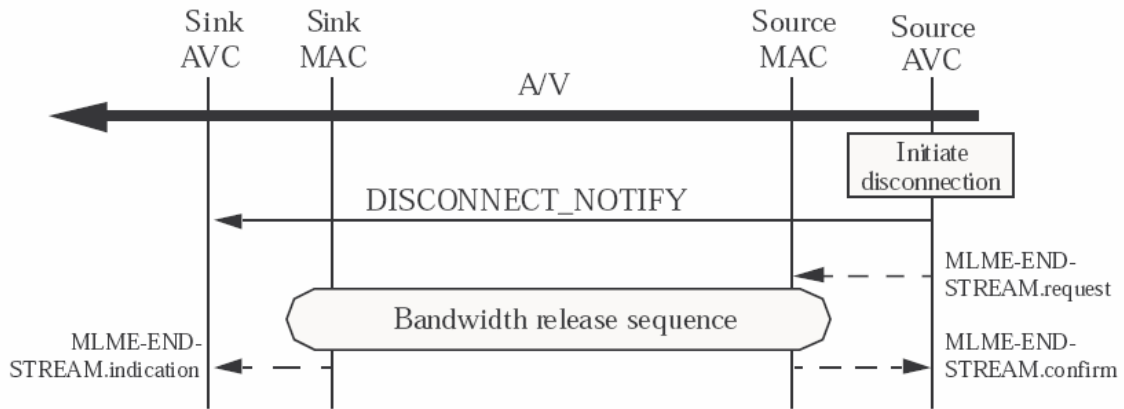
Figure 34: Message sequence for a Source initiated disconnection procedure
