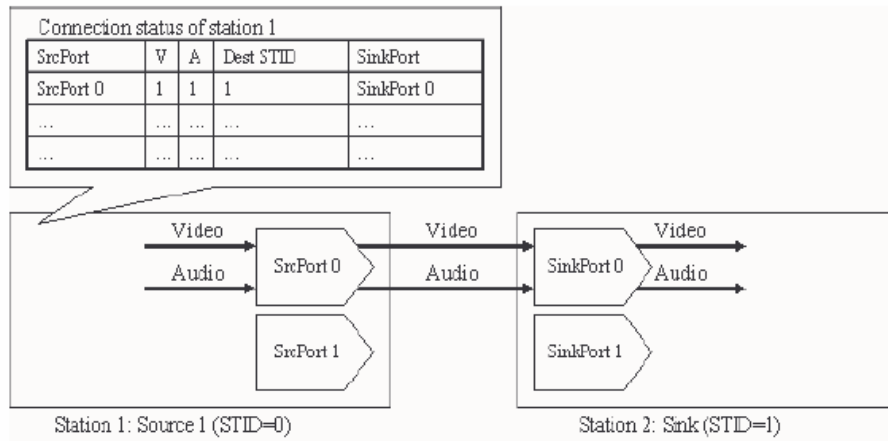
Figure 37: Example of A/V transmission procedure
