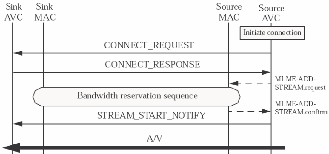
Figure 31: Message sequence for source initiated connection
