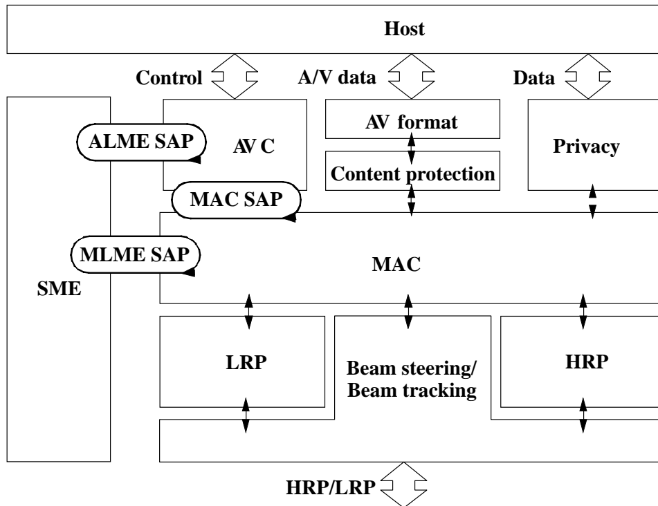
Figure 3: Reference model for WirelessHD specification
