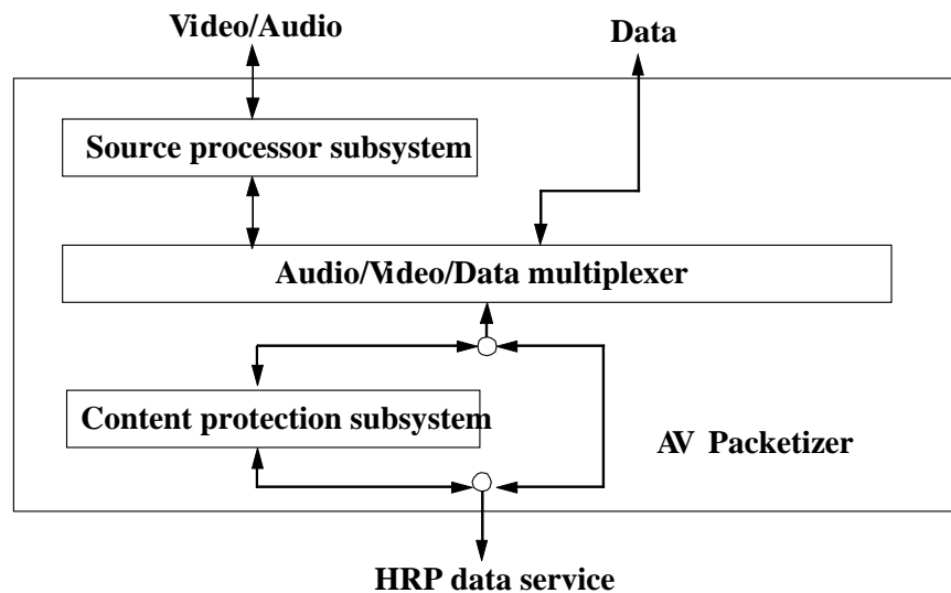
Figure 39: Reference model of A/V packetizer
