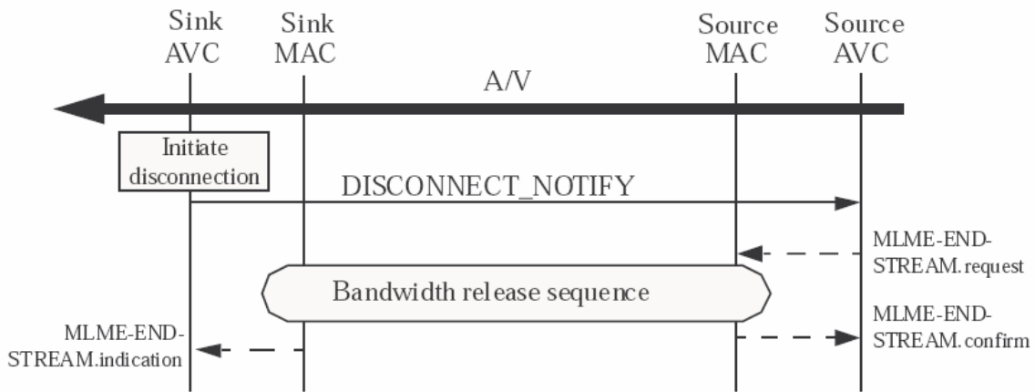
Figure 35: Message sequence for Sink initiated disconnection
