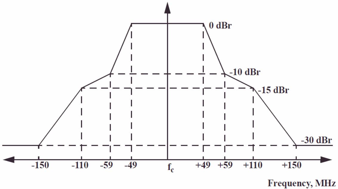
Figure 13: LRP TX mask
